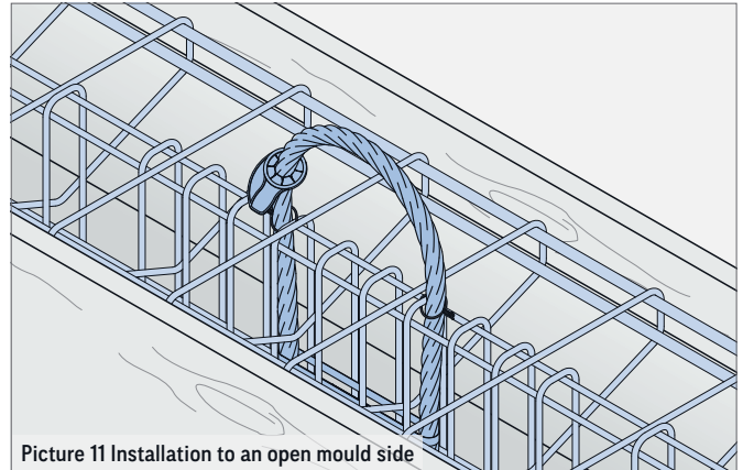
Picture 11 Installation to an open mould side
